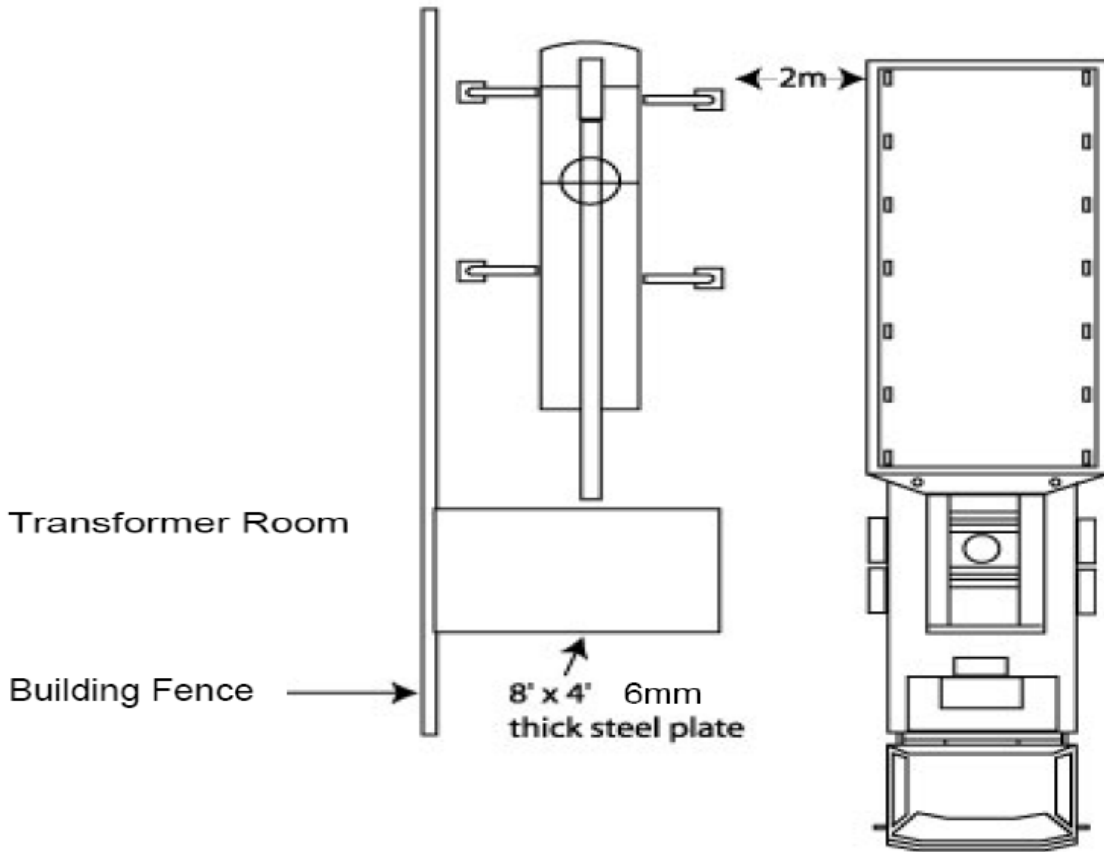
Fig. 4 Plan view of Crane and Trailer
