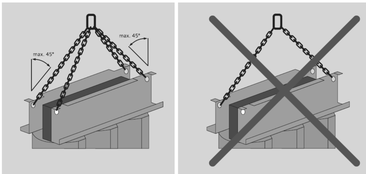
Fig. 2 Lifting lugs
