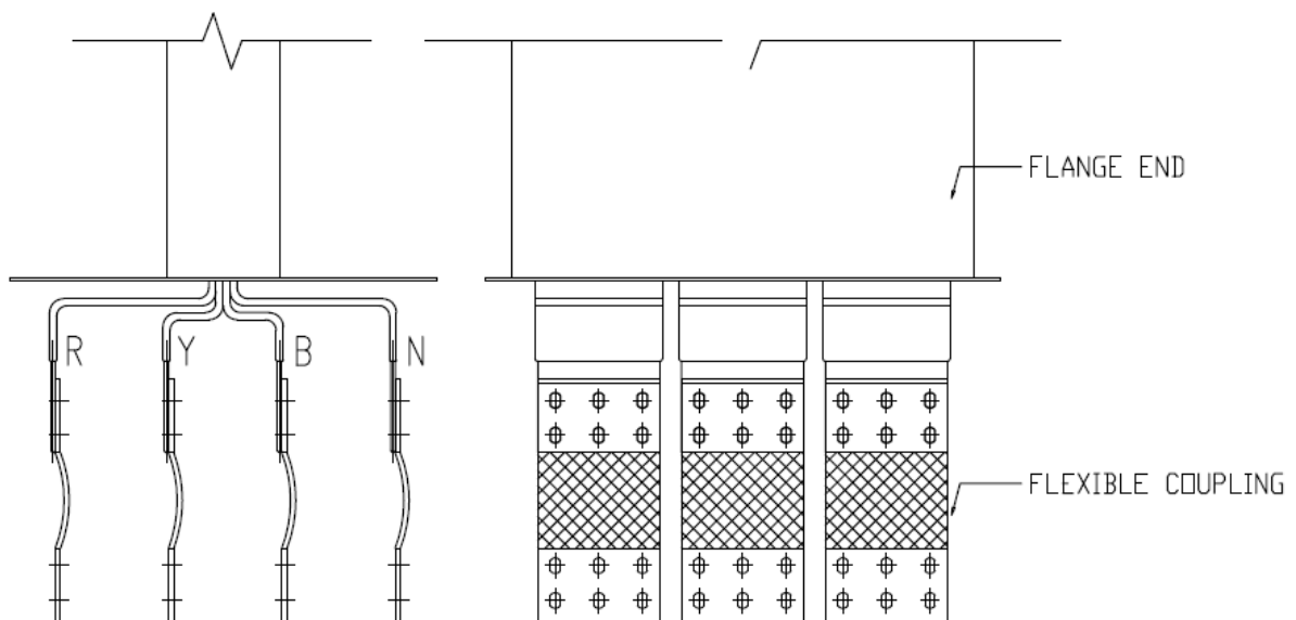
Installation Detail 3: Flange end & flexible coupling
